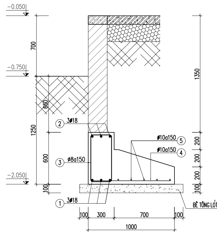
MÓNG MB.3
